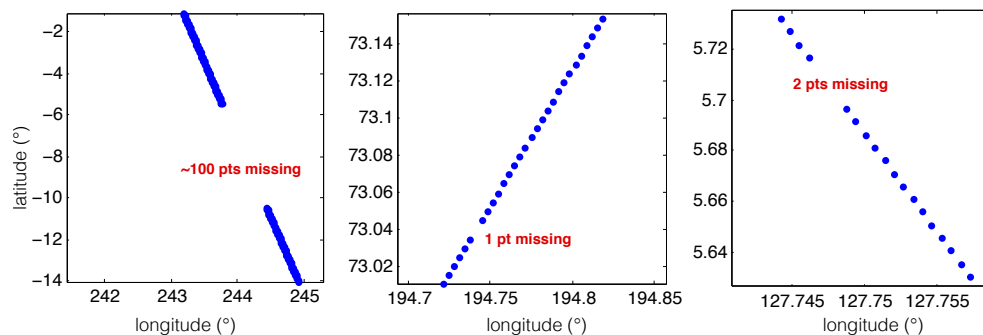
Figure 4. A few examples of irregularly-spaced points in the MOLA database.
