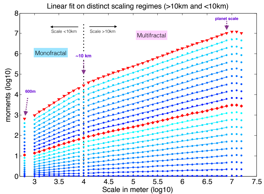
Figure 2. Linear fit on the two different scaling regimes (inferior and superior to 10 km) for every 21 statistical moments from 0.1 to 2. The color code is the same as in Fig. 1. Quantities on that plot are scaling according to the moment scaling function \xi(q) .
