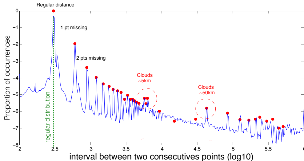
Figure 5. Comparison between effective irregularities in the MOLA database and artificial irregularities on simulations. Irregularities are expressed as a proportion of occurrences from the maximum possible in log10 space (0 means all fluctuations are observed). The blue line represents the effective irregularity of actual data. Red points are obtained from the synthetic irregularities on multifractal simulations. The good agreement between maxima of the blue curve and red points indicates that effective irregularity is accurately reproduced by simulations.
